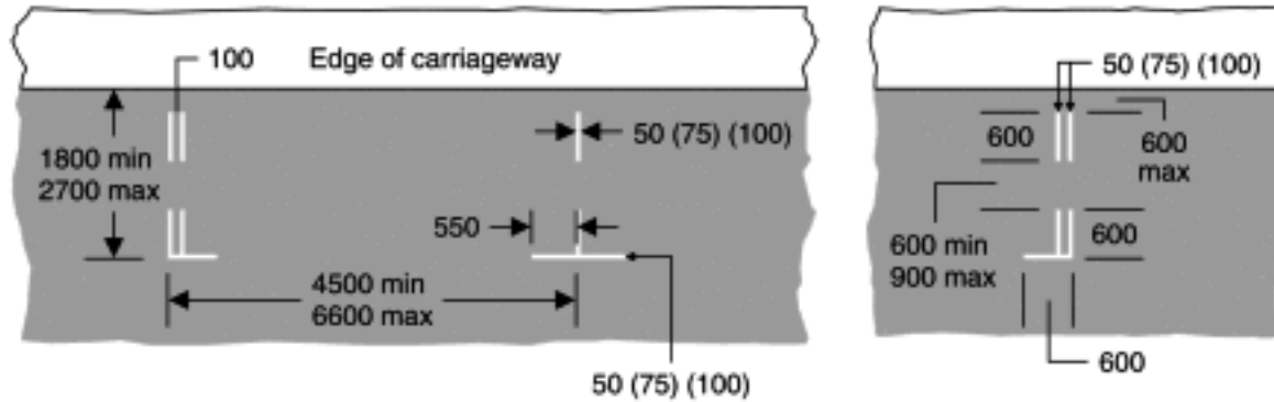
Parking bay marked with individual parking spaces (Longitudinal marking)
